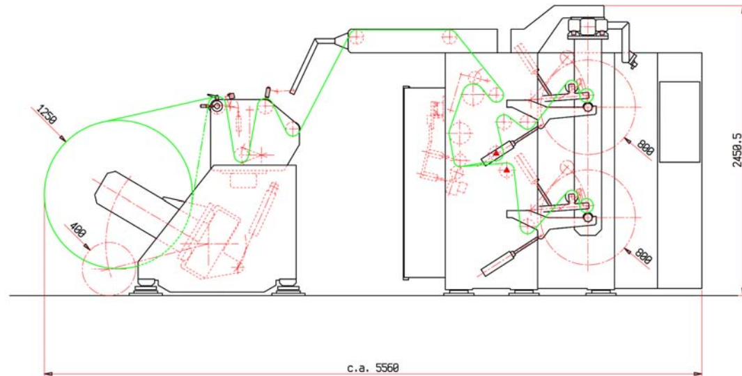
Automatic set-up
