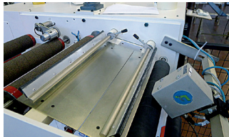
Splicing table.
